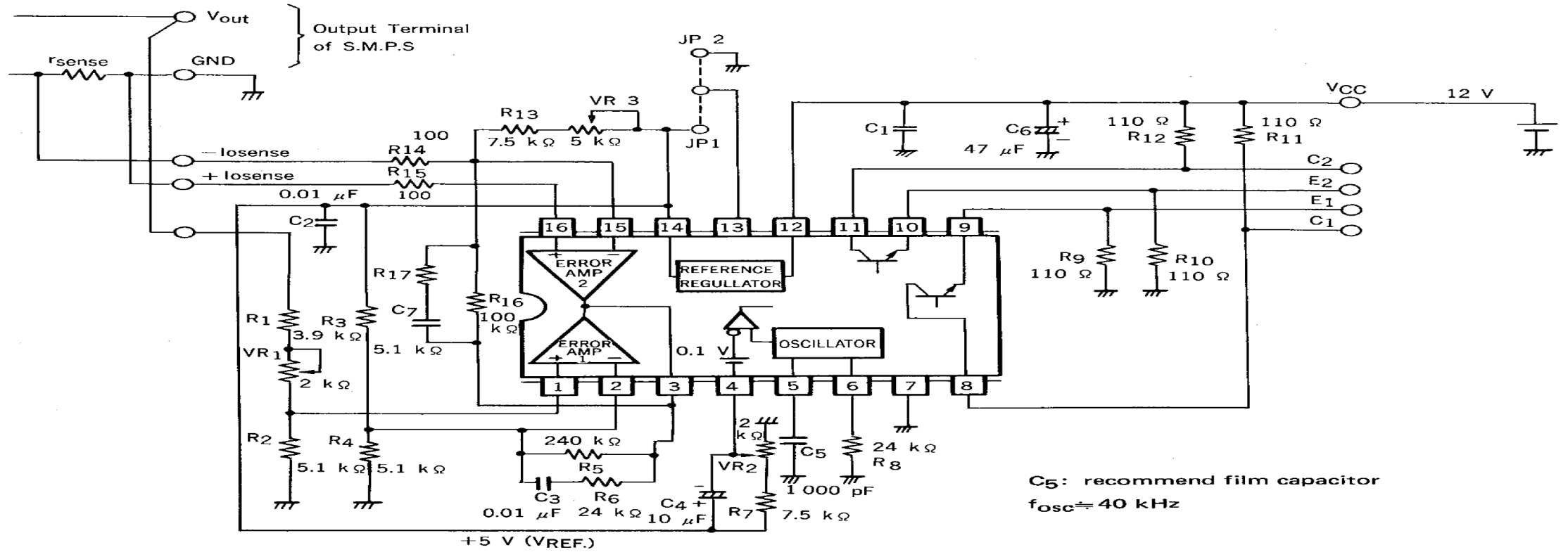
Fig. 2 Circuit
